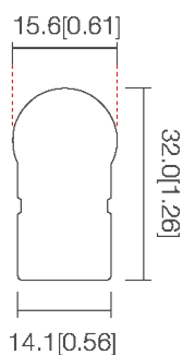
Sectional View
